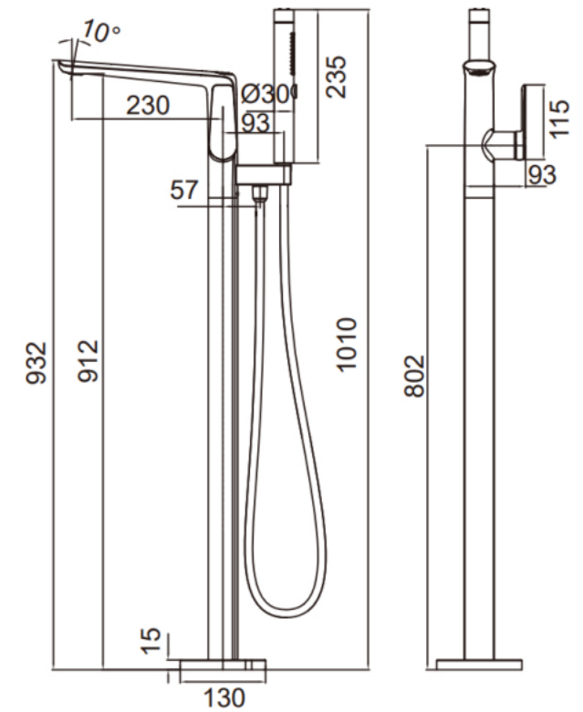
DC10280 Freestanding Bathtub Faucet Finishing: Brushed Gold
