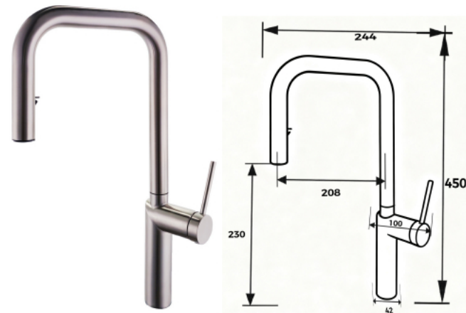
DCSSKT0009 Kitchen Mixer Finishing: Brushed Material: 304 Stainless Steel
