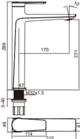
DC10272-5 Basin Mixer Finishing: Brushed Nickel Material: Brass
