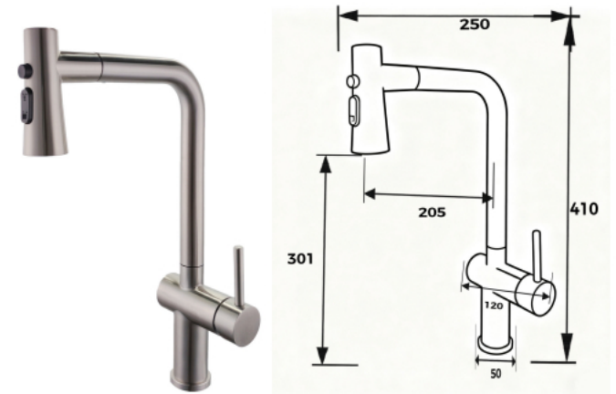
DCSSKT0007 Kitchen Mixer Finishing: Brushed Material: 304 Stainless Steel
