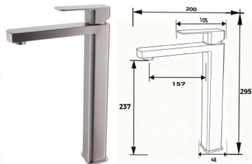
DCSS0006A Basin Mixer Finishing: Brushed Material: 304 Stainless Steel
