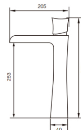
DC10045-3A Basin Mixer Finishing: Gun Grey Material: Brass
