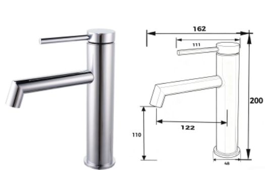
DCSS0006 Basin Mixer Finishing: Brushed Material: 304 Stainless Steel
