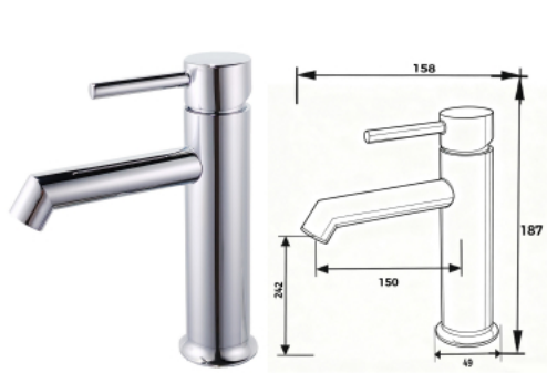
DCSS0007 Basin Mixer Finishing: Brushed Material: 304 Stainless Steel
