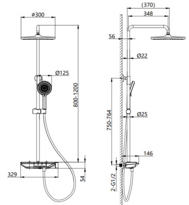
DC10237 Shower Mixer Finishing: Chrome Material: Plastic
