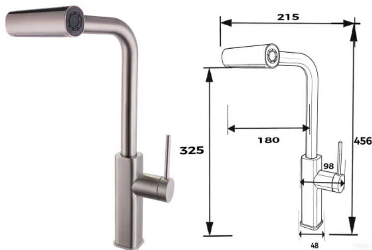
DCSSKT0011 Kitchen Mixer Finishing: Brushed Material: 304 Stainless Steel
