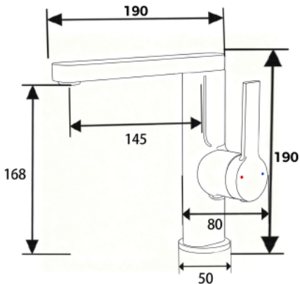
DC10085 Basin Mixer Finishing: Chrome Material: Brass
