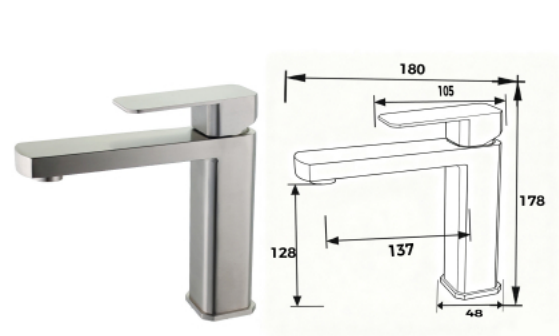
DCSS0006 Basin Mixer Finishing: Brushed Material: 304 Stainless Steel
