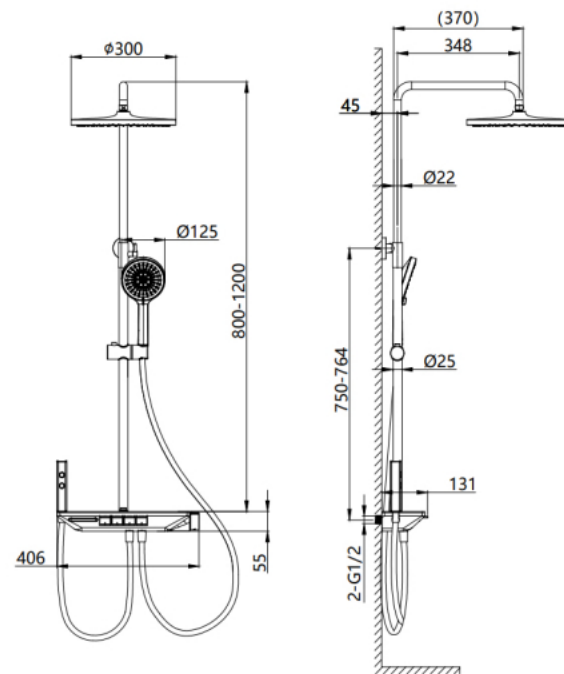
DC10239 Shower Mixer Finishing: Chrome Material: Plastic
