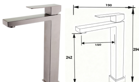
DCSS0007A Basin Mixer Finishing: Brushed Material: 304 Stainless Steel
