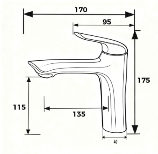
DC10087 Basin Mixer Finishing: Chrome Material: Brass
