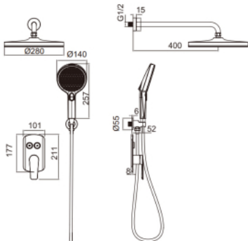
DC10278 Shower Mixer Finishing:
