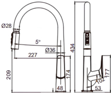
DC10038 Kitchen mixer Finishing: Black
