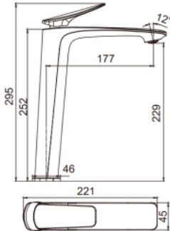
DC10037 Basin mixer(tall) Finishing: Black
