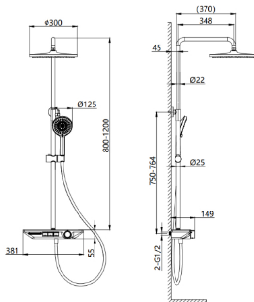
DC10240 Shower Mixer Finishing: Chrome Material: Plastic
