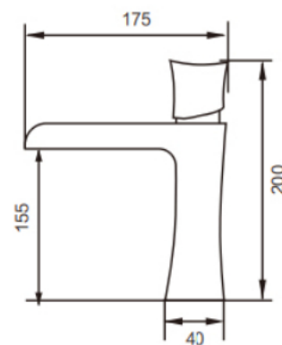
DC10045-3 Basin Mixer Finishing: Gun Grey Material: Brass
