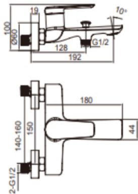
DC10275-6 Shower Mixer Finishing: Rose Gold Material: Brass
