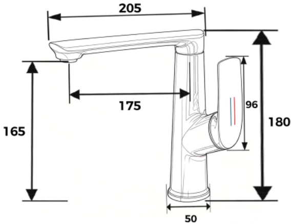
DC10087 Basin Mixer Finishing: Cream Material: Brass
