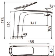
DC10036 Basin mixer Finishing: Black
