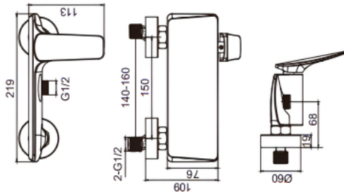
DC10040 Shower Kit Finishing: Black
