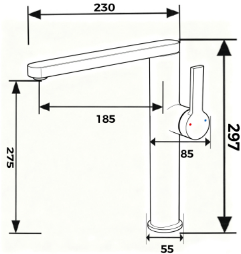
DC10086 Basin Mixer Finishing: Chrome Material: Brass
