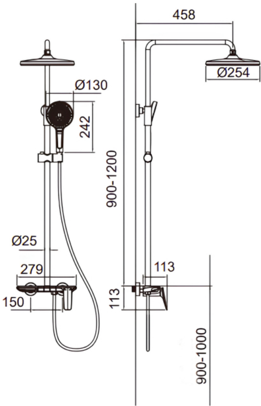
DC10042 Shower Kit Finishing: Black
