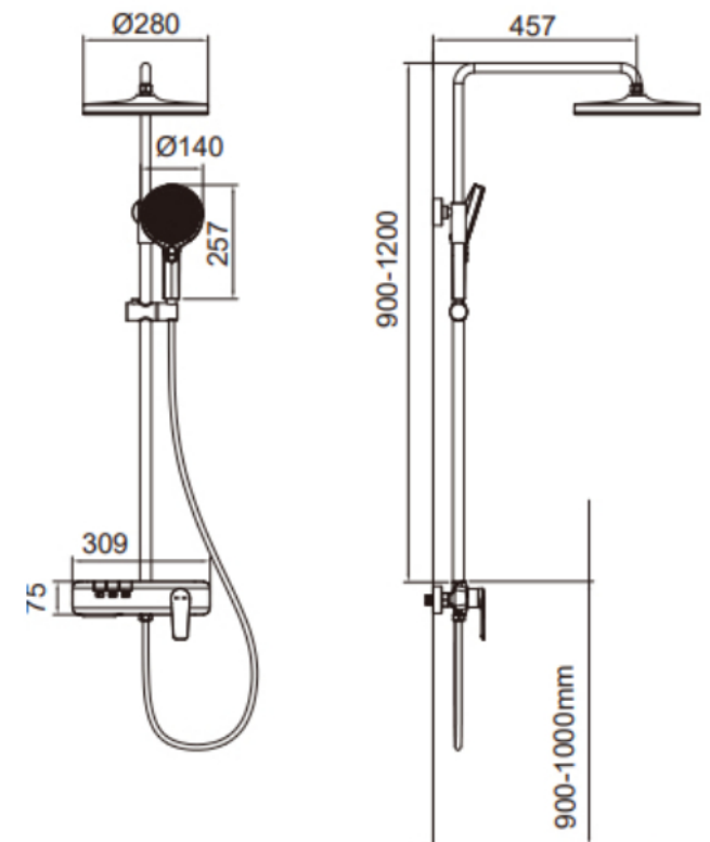
DC10268 Shower Mixer Finishing: Brushed Gold Material: Brass
